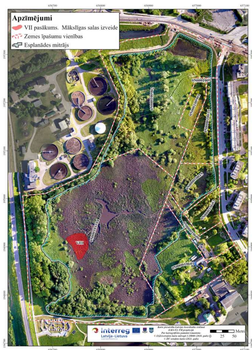
Figure 65. Location of the planned artificial island in the Esplanade Wetland
