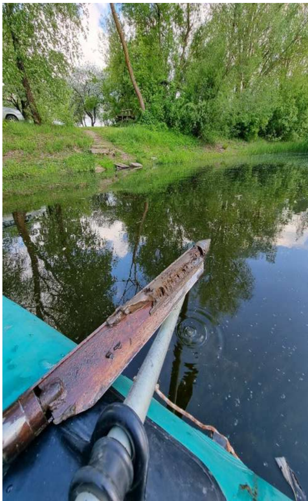
Figure 106. Measuring thickness of accumulated sludge (Photo: A. Balevičius)
